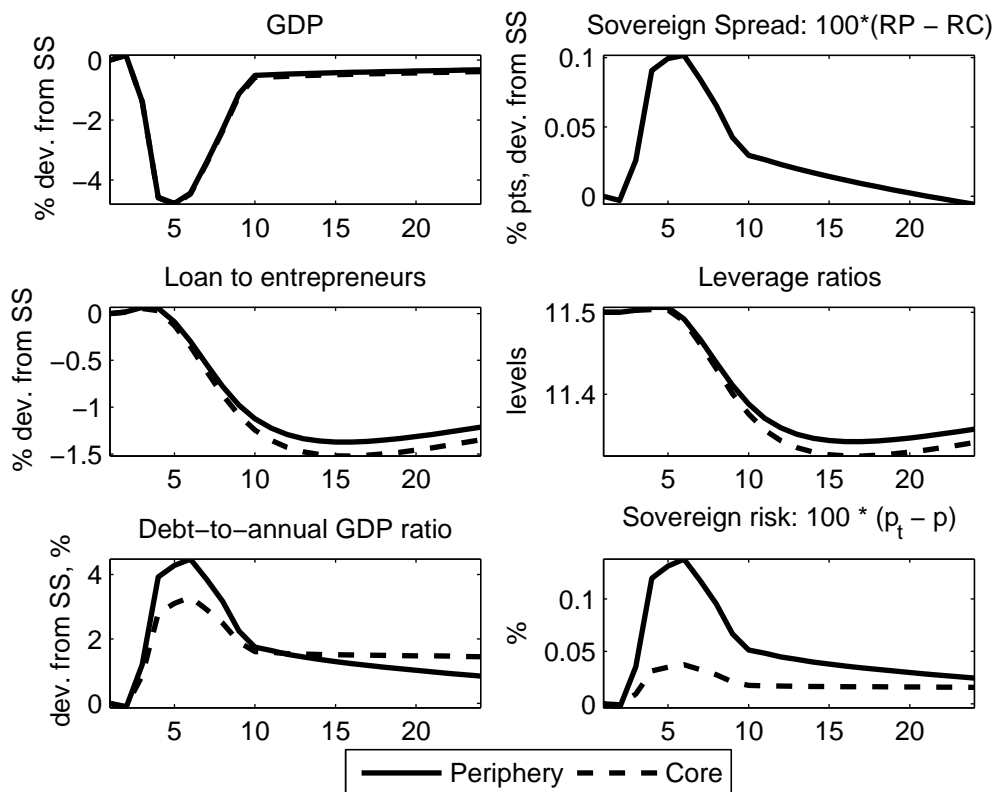
Figure 1: Benchmark Simulation. Negative TFP shocks without Central Bank Intervention.
